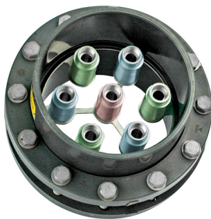
8" System with flange
